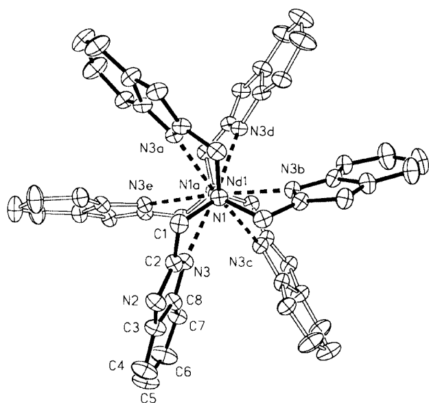
Fig. 1 Top view of the cation [\text{Nd}(\text{ntb})_2]^{3+} ( \Lambda configuration) in complex 5 showing atoms as thermal ellipsoids at 30% probability level. All H atoms have been omitted for clarity.
