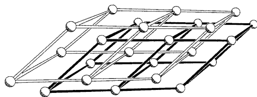
Fig. 6 Twofold interpenetration of \alpha -polonium-related nets in complex 6 . The balls represent Nd atoms, and each rod represents a pair of 2-benzimidazolymethyl arms and a bpen spacer that are connected by hydrogen bonds.
